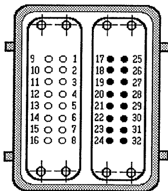
Figure 1: Plug on the handling device
