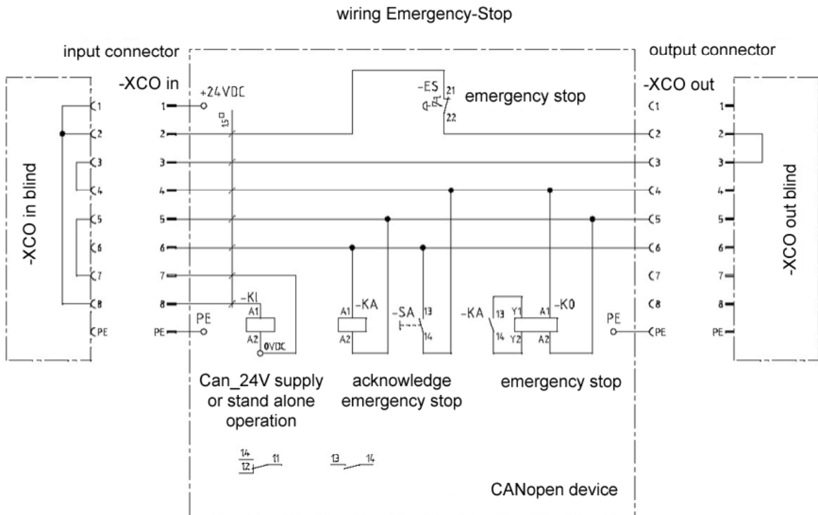
Figure 8 — Emergency-stop wiring
